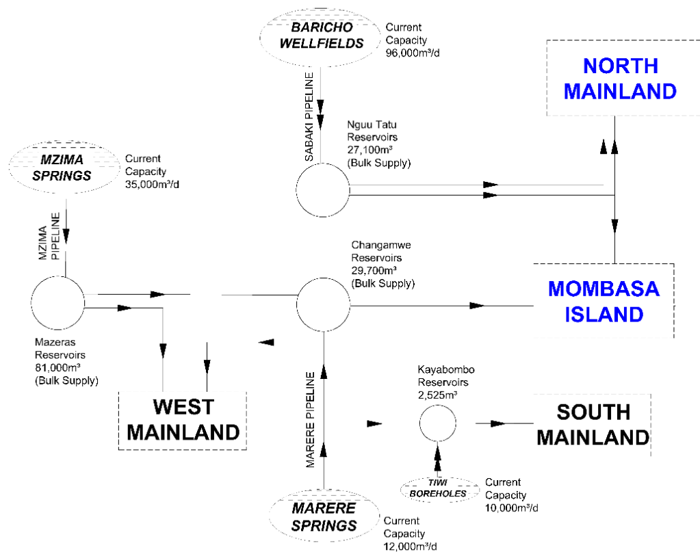
Figure 1: Schematic of Existing Water Supply System in Mombasa
